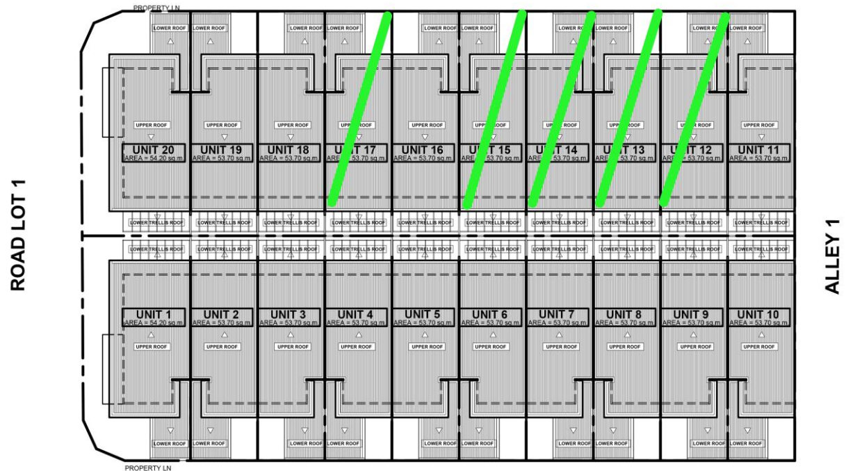
DURHAM ROWS SITE DEVELOPMENT PLAN SCALE 1:250 MTS
